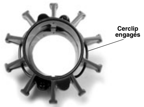
Figure 17 – Cerclip engagés
