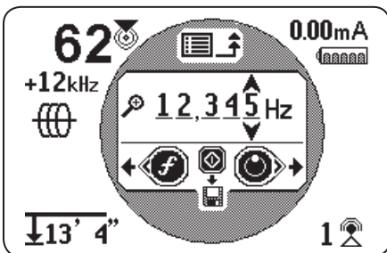
Figure 12 – Frequency Input screen
