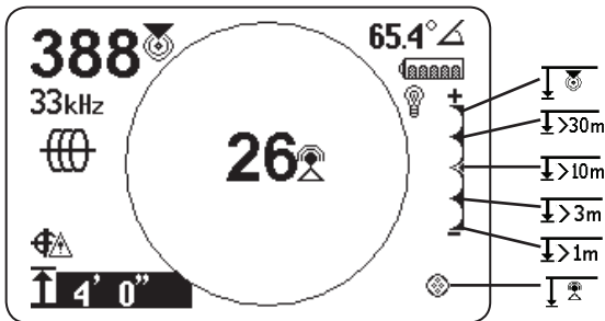
Figure 15 – Proximity Threshold Control limit set to display Signal Strength
