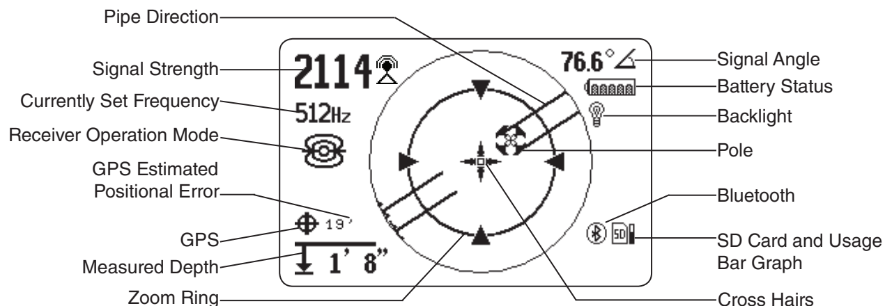
Figure 2 – Sonde Mode Display Example
