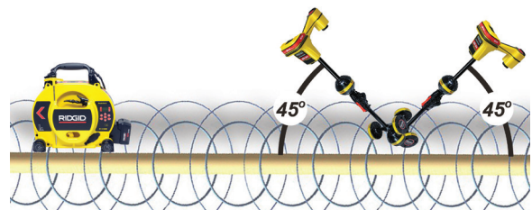
Figure 5 – 45° tilt test
