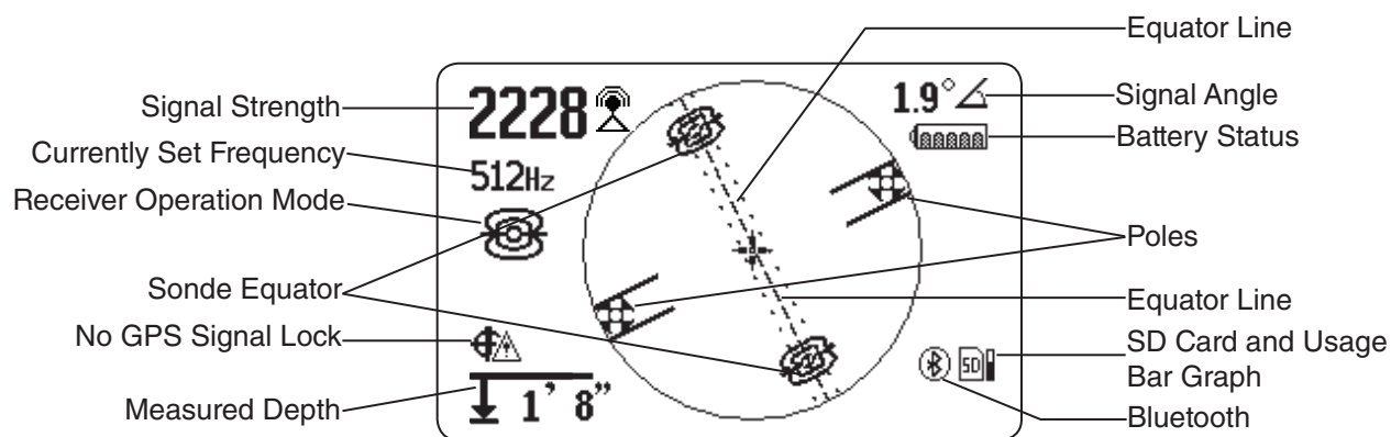
Figure 3 – Display showing Equator Line and Equator Sonde Icons
