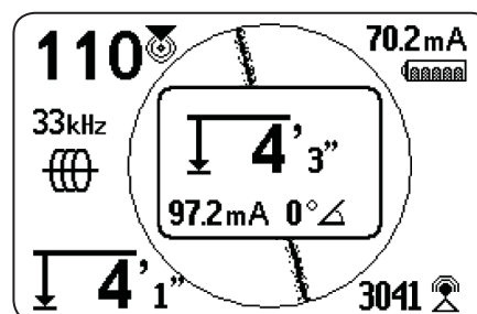
Figure 10 – Depth Average Report
