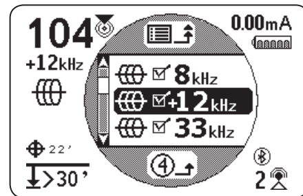
Figure 13 – Active custom frequency
