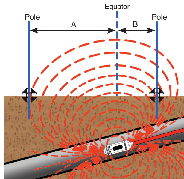
Figure 9 – Tilted RIDGID NaviTrack Battery Sonde
