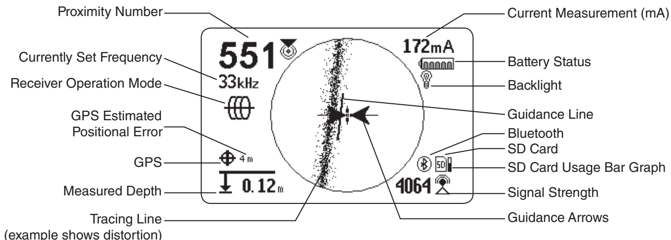
Figure 1 – Line Trace Mode Display Example
