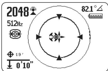
Figure 6 – Centering Pole on the Cross Hairs
