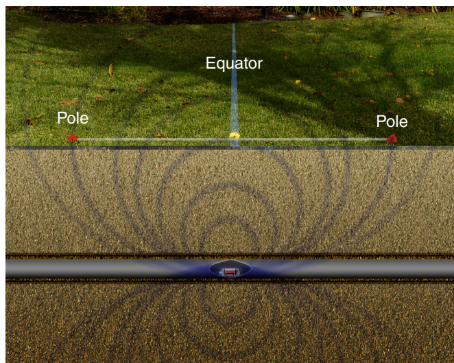
Figure 7 – Position of the Poles and the Equator
